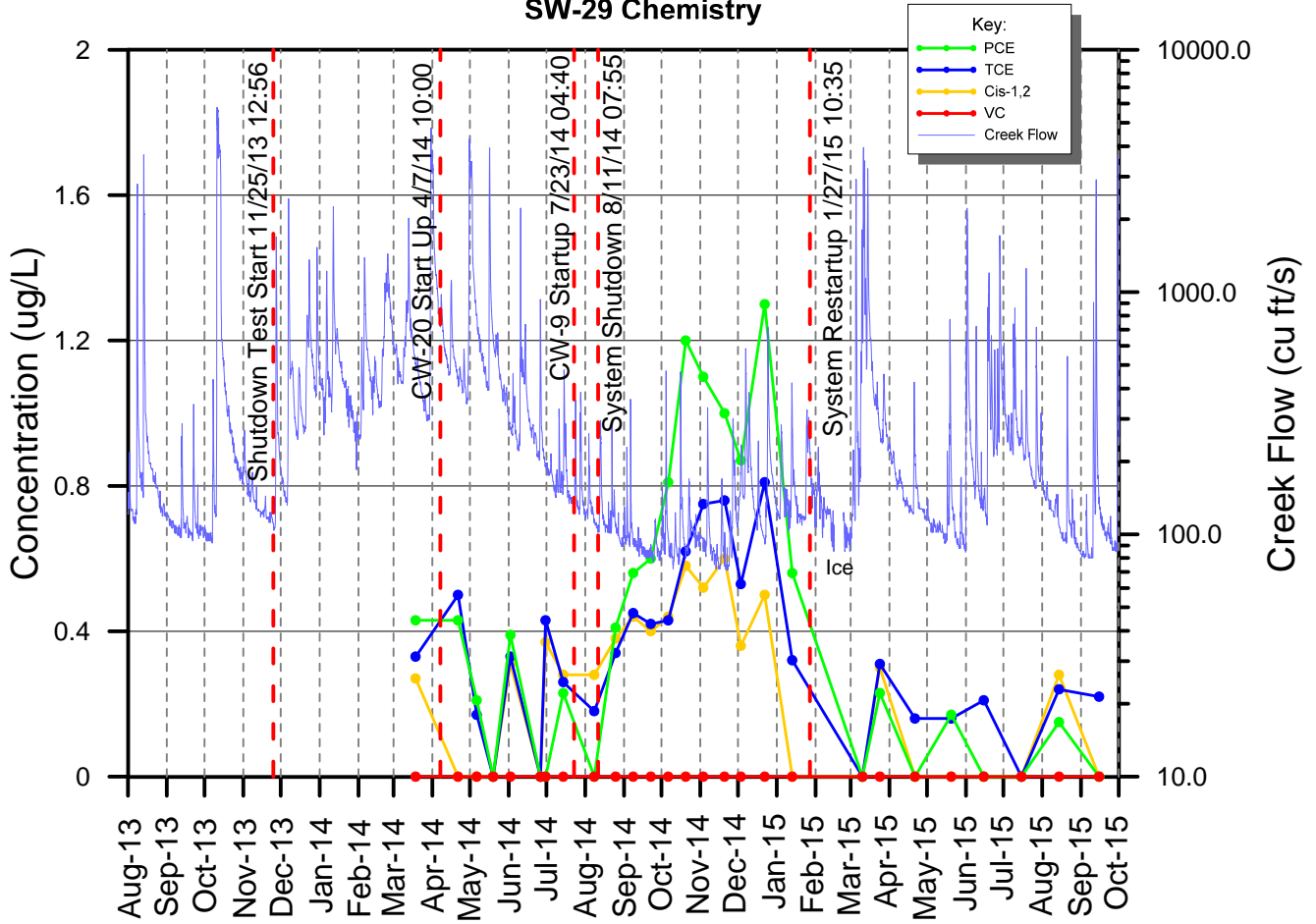
Figure 3.5-17 SW-29 Chemistry
